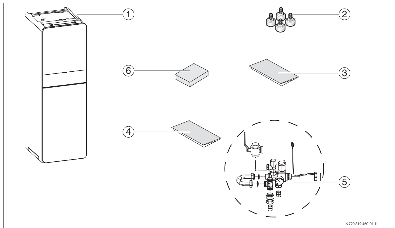
Fig. 1 Standardleverance
